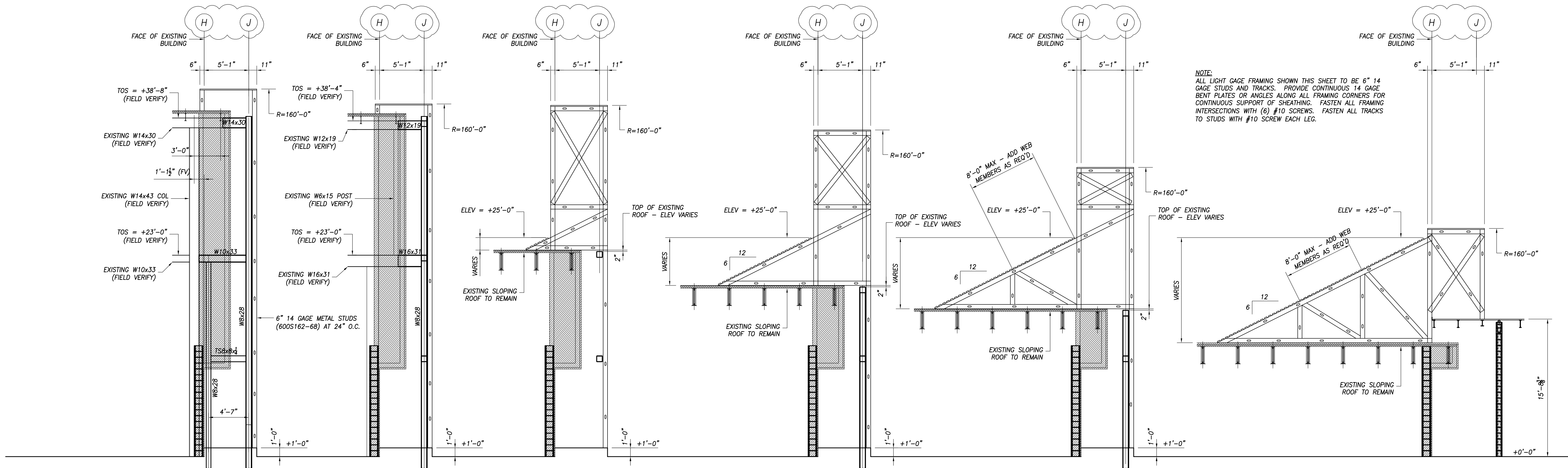
FRAMING ELEVATION 1 3/16" = 1'-0"
